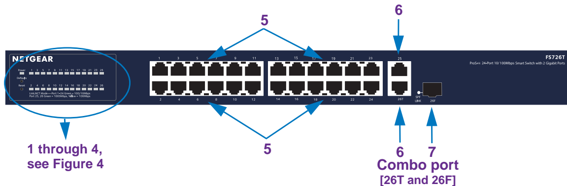
Figure 3. Front panel
