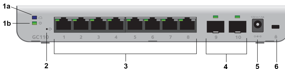
Figure 2. Back panel model GC110
