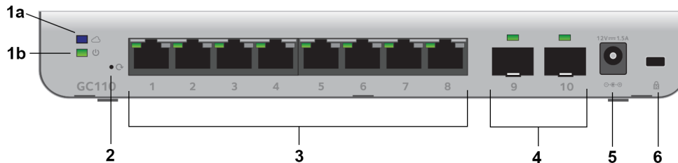
Figure 2. Back panel model GC110
