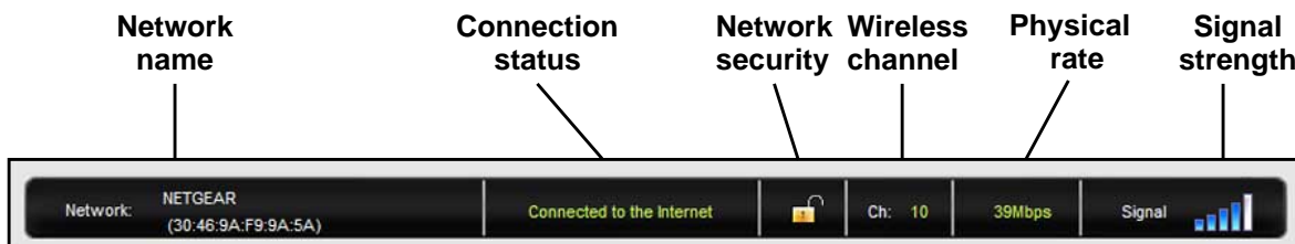
Figure 1. Status bar
