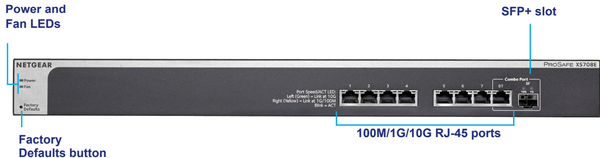
Figure 2. Switch front panel
