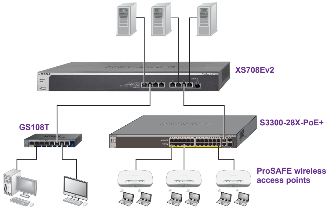
Figure 5. Backbone switching configuration
